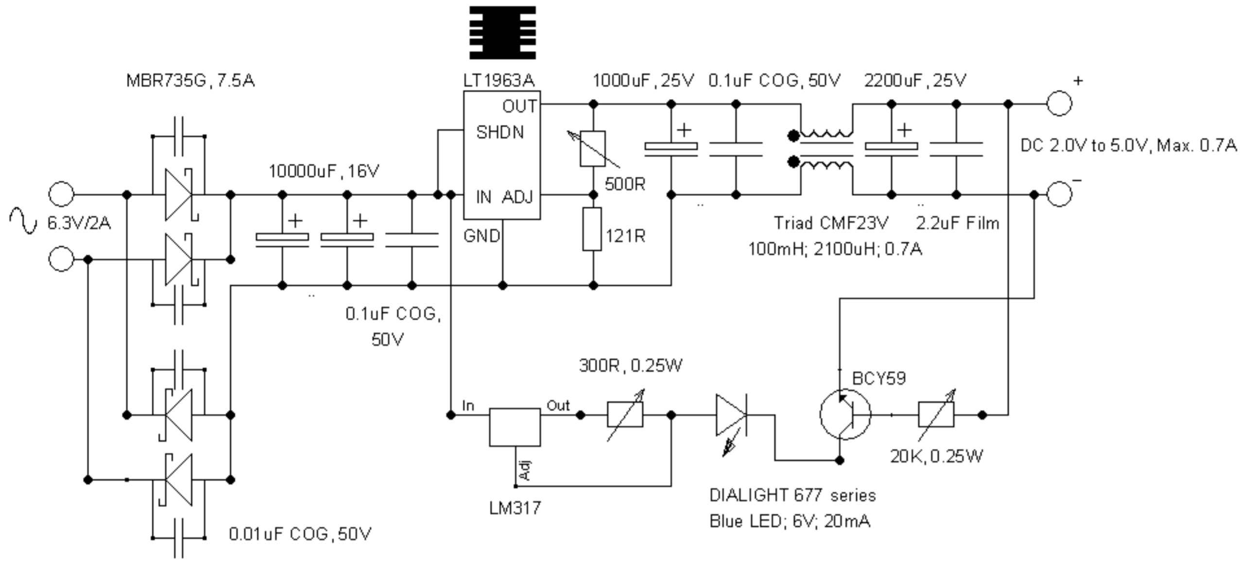
LED INDICATOR CIRCUIT
